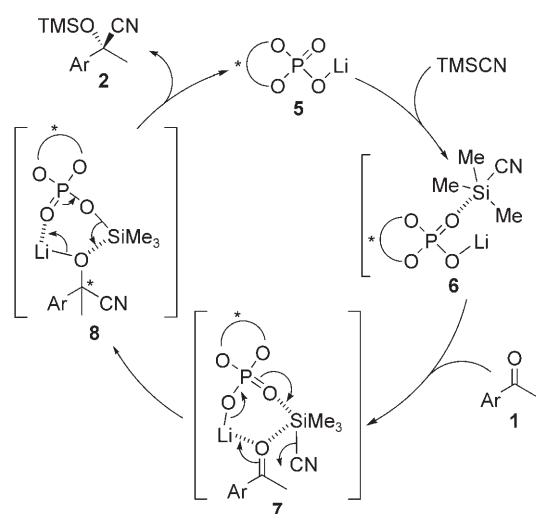
Figure 2. Postulated catalytic cycle with a Lewis acid–base conjugate catalyst.
