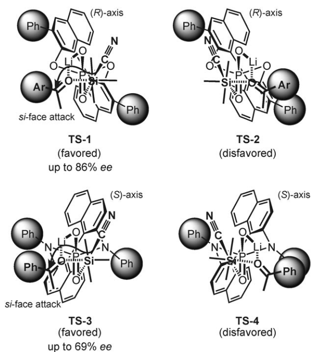
Figure 3. Possible transition states.
