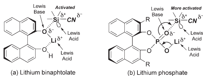
Figure 1. Design of chiral lithium phosphate complexes as Lewis acid–base conjugate catalysts.
